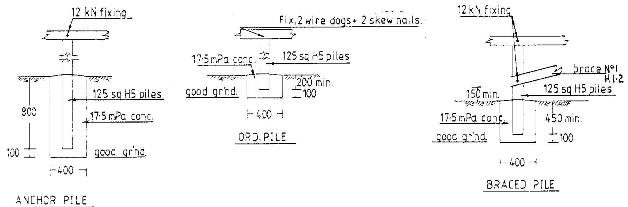
DETAIL FOR 125 sq PILES
